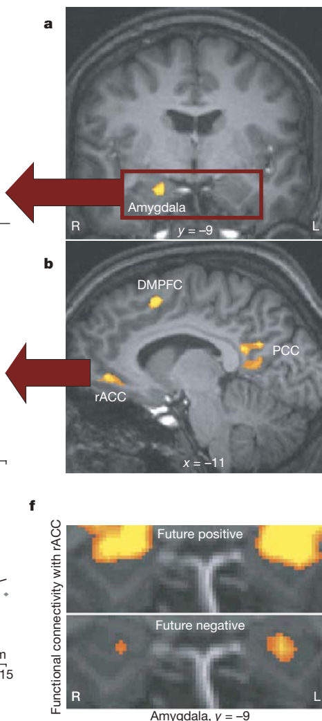
Figure 2 | Activity in the amygdala and rACC and its relation to optimism. ROIs defined by contrasting all trials with fixation (shown at P < 0.0005 , uncorrected) reveal activity of a , the amygdala (Talarich coordinates of peak voxel: 20, -9, -14) and b , the rACC (Brodmann Area (BA) 32: -11, 42, -1), the PCC (BAs 30 and 31: -4, -47, 19) and the dorsal medial prefrontal cortex (DMPFC; BA 6: -8, 12, 52). BOLD signals in both c , the amygdala and d , the rACC reduced while imagining negative future events. e , BOLD signal in the rACC during future positive events versus future negative events correlated with trait optimism ( -9, 39, -2 ; r = 0.5 , P < 0.05 ). f , Functional connectivity map with rACC as the seed reveals extensive correlation with the amygdala signal during future positive trials, and restricted correlation during future negative trials. The red square in a indicates the region shown in f . N = 15 ; error bars, \pm s.e.m.; * P < 0.05 .
